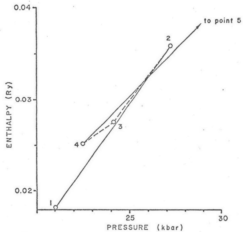
FIG. 2. Cs enthalpy.
